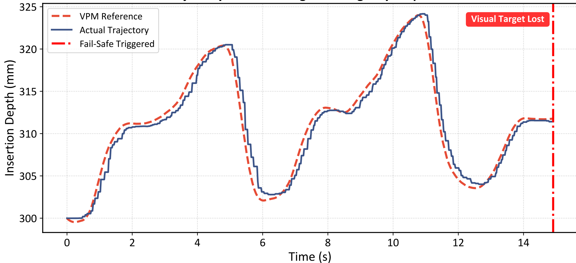
Trajectory Profile during an Emergency Stop Event
